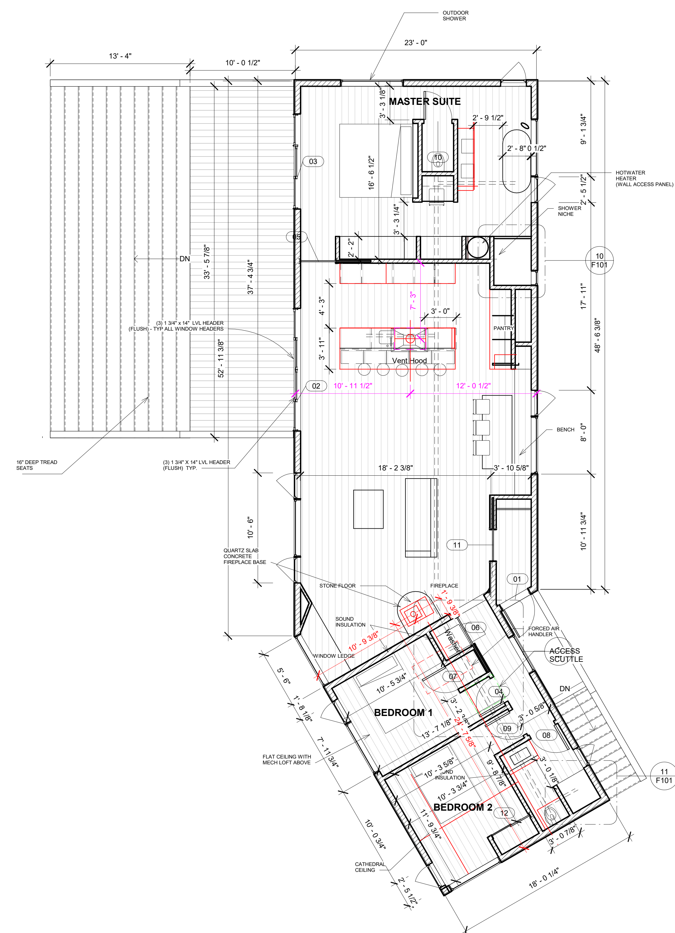
1 FIRST FLOOR FRAMING PLAN 3/16" = 1'-0"
